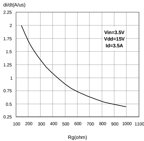
Figure 30. Turn On Current Slope
